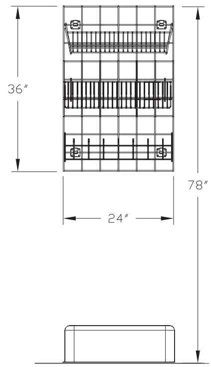
FRONT ELEVATION
