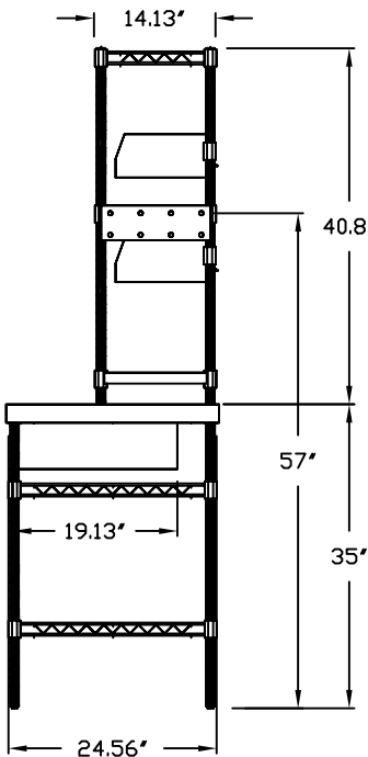
SIDE ELEVATION
