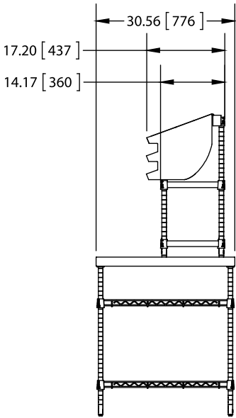
SIDE ELEVATION
