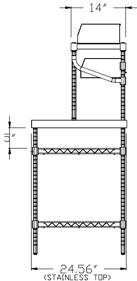
SIDE ELEVATION
