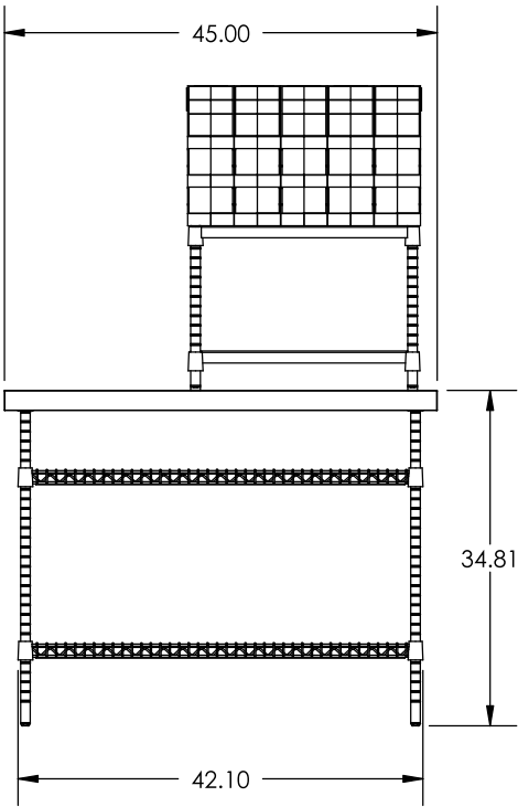
FRONT ELEVATION
