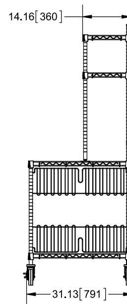
SIDE ELEVATION
