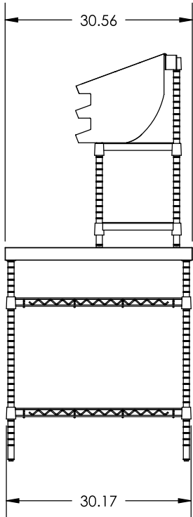
SIDE ELEVATION
