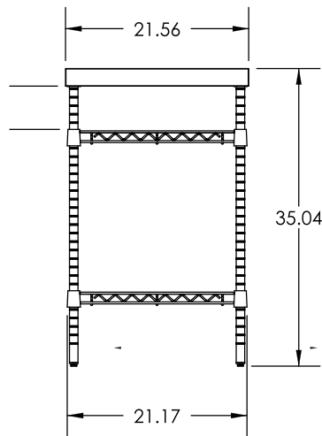
SIDE ELEVATION
