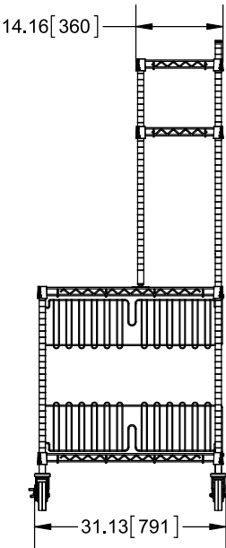
SIDE ELEVATION
